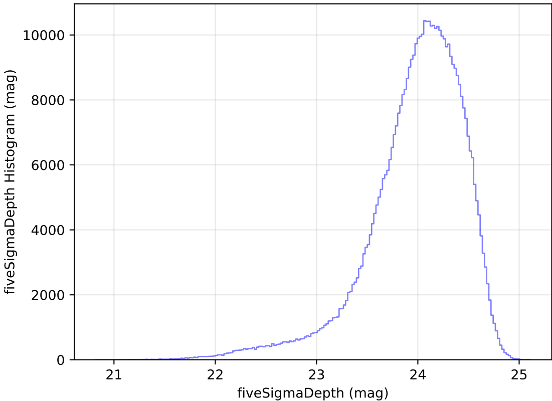
ddf_loaded_half_fl4_v3.4_10yrs r: fiveSigmaDepth Histogram
