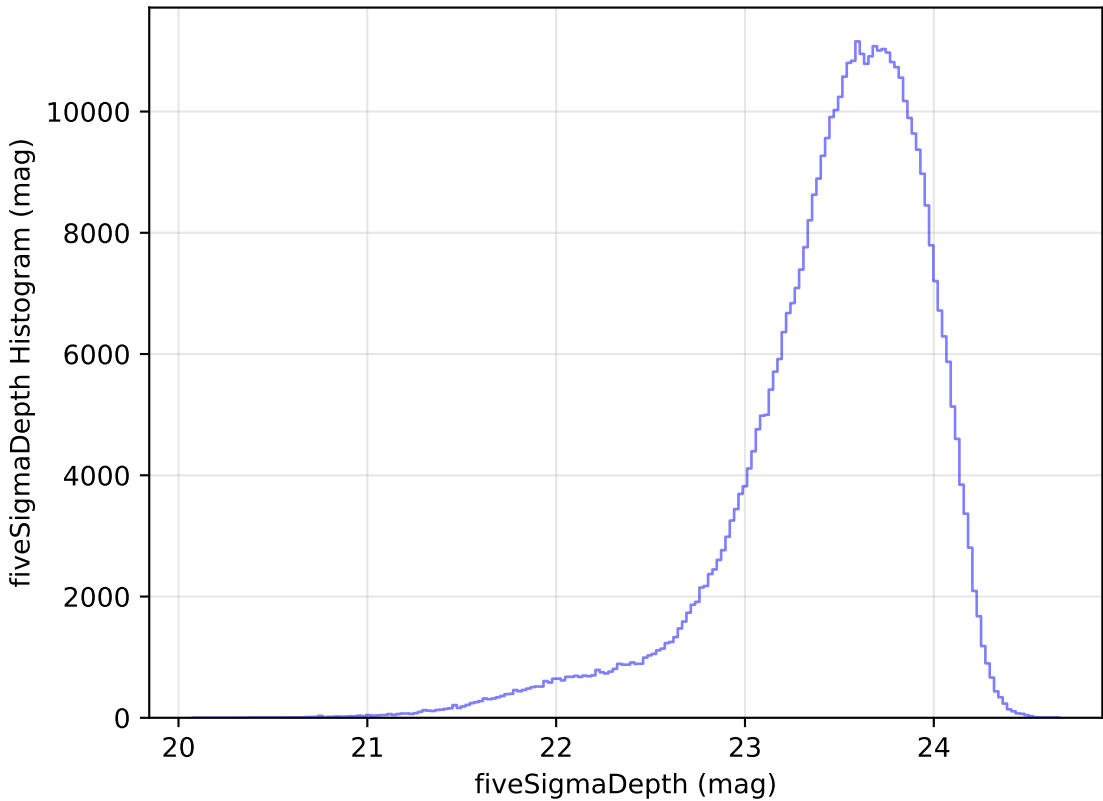
ddf_loaded_half_fl4_v3.4_10yrs i: fiveSigmaDepth Histogram
