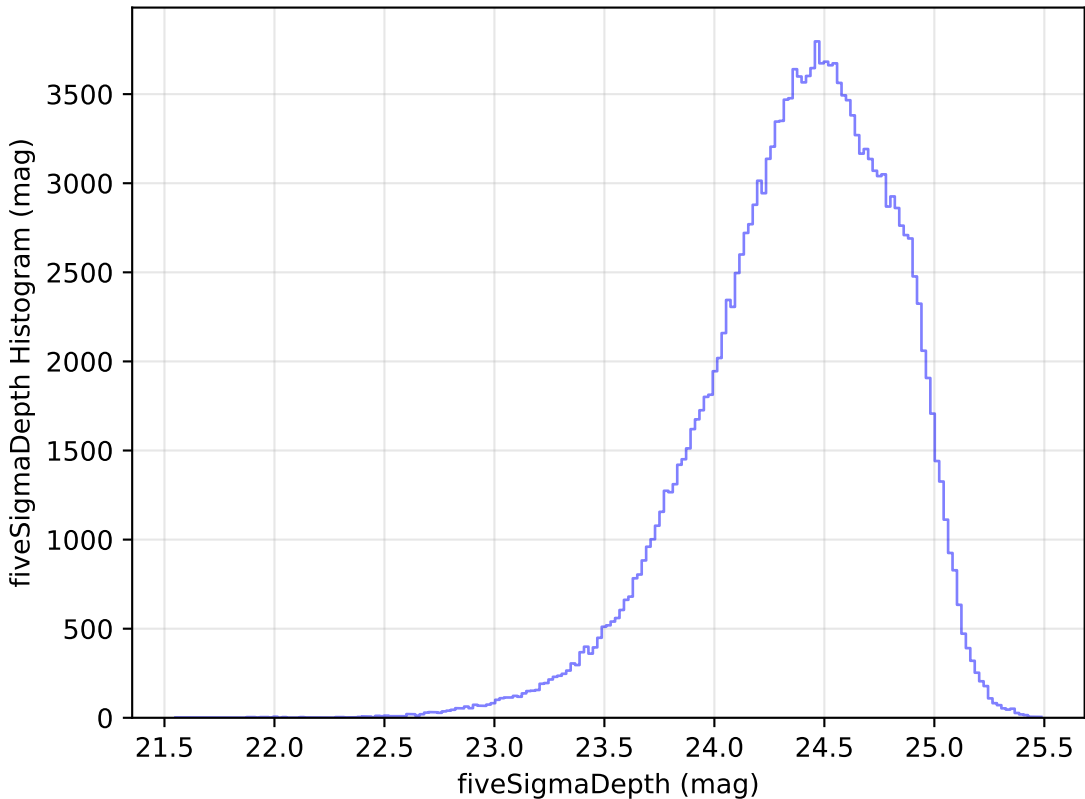
ddf_loaded_half_fl4_v3.4_10yrs g: fiveSigmaDepth Histogram
