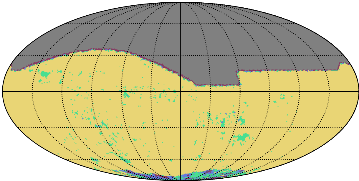
ddf_loaded_half_fl4_v3.4_10yrs i band: YearCoverage night
