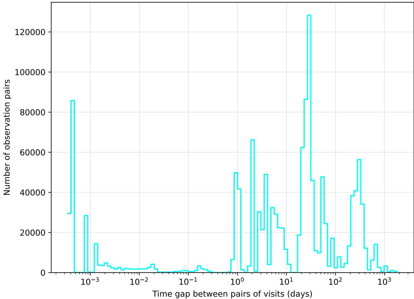
ddf_loaded_half_fl4_v3.4_10yrs u band: Tgaps observationStartMJD
