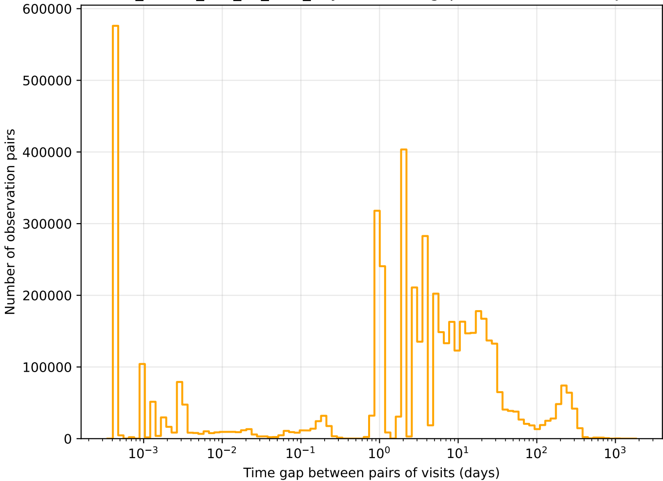
ddf_loaded_half_fl4_v3.4_10yrs r band: Tgaps observationStartMJD
