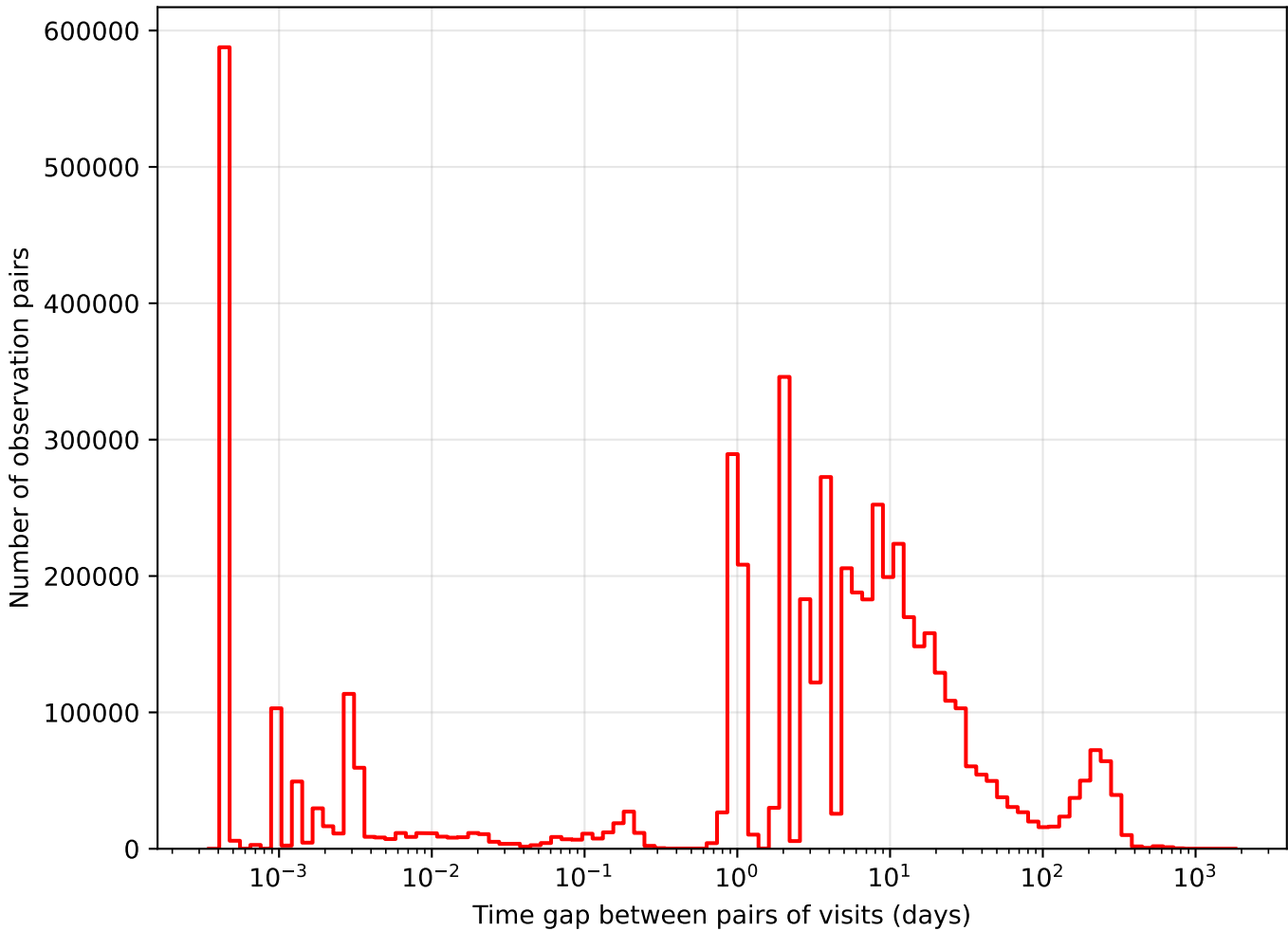
ddf_loaded_half_fl4_v3.4_10yrs i band: Tgaps observationStartMJD
