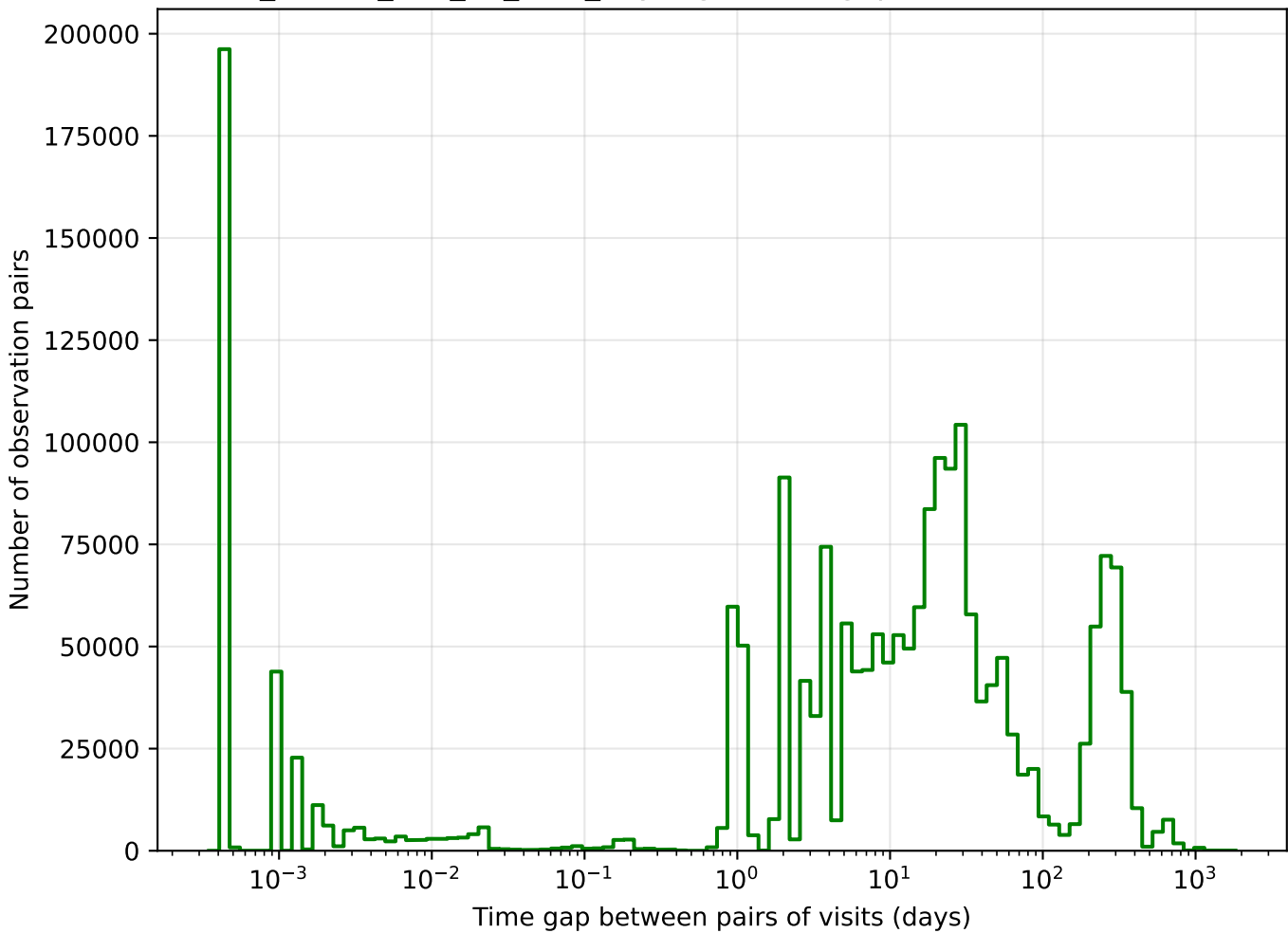
ddf_loaded_half_fl4_v3.4_10yrs g band: Tgaps observationStartMJD
