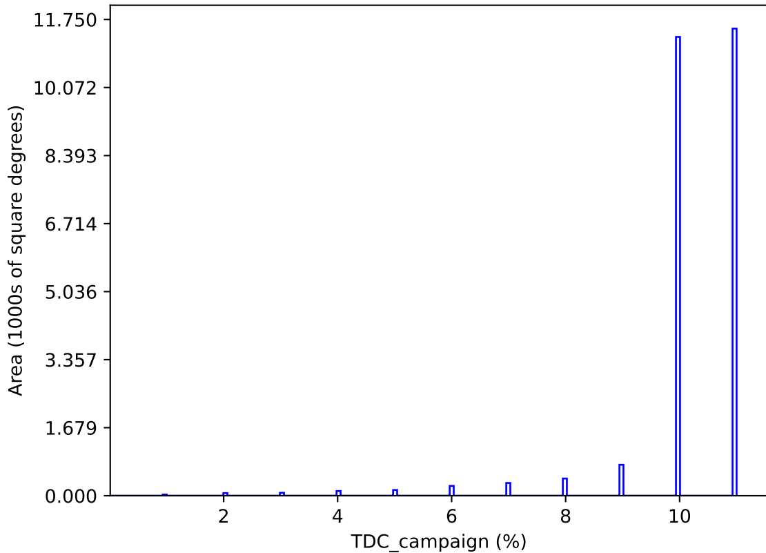
ddf_loaded_half_fl4_v3.4_10yrs : TDC_campaign
