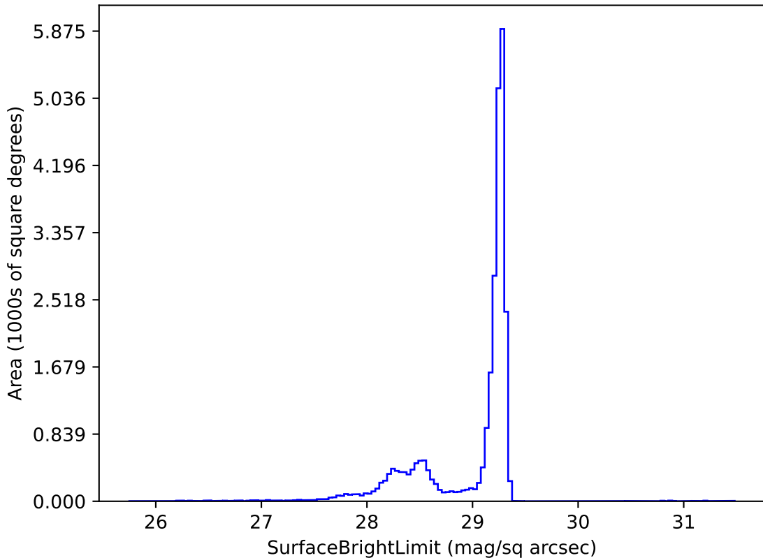
ddf_loaded_half_fl4_v3.4_10yrs z: SurfaceBrightLimit
