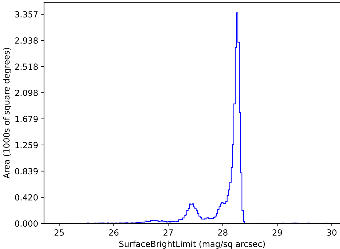
ddf_loaded_half_fl4_v3.4_10yrs y: SurfaceBrightLimit
