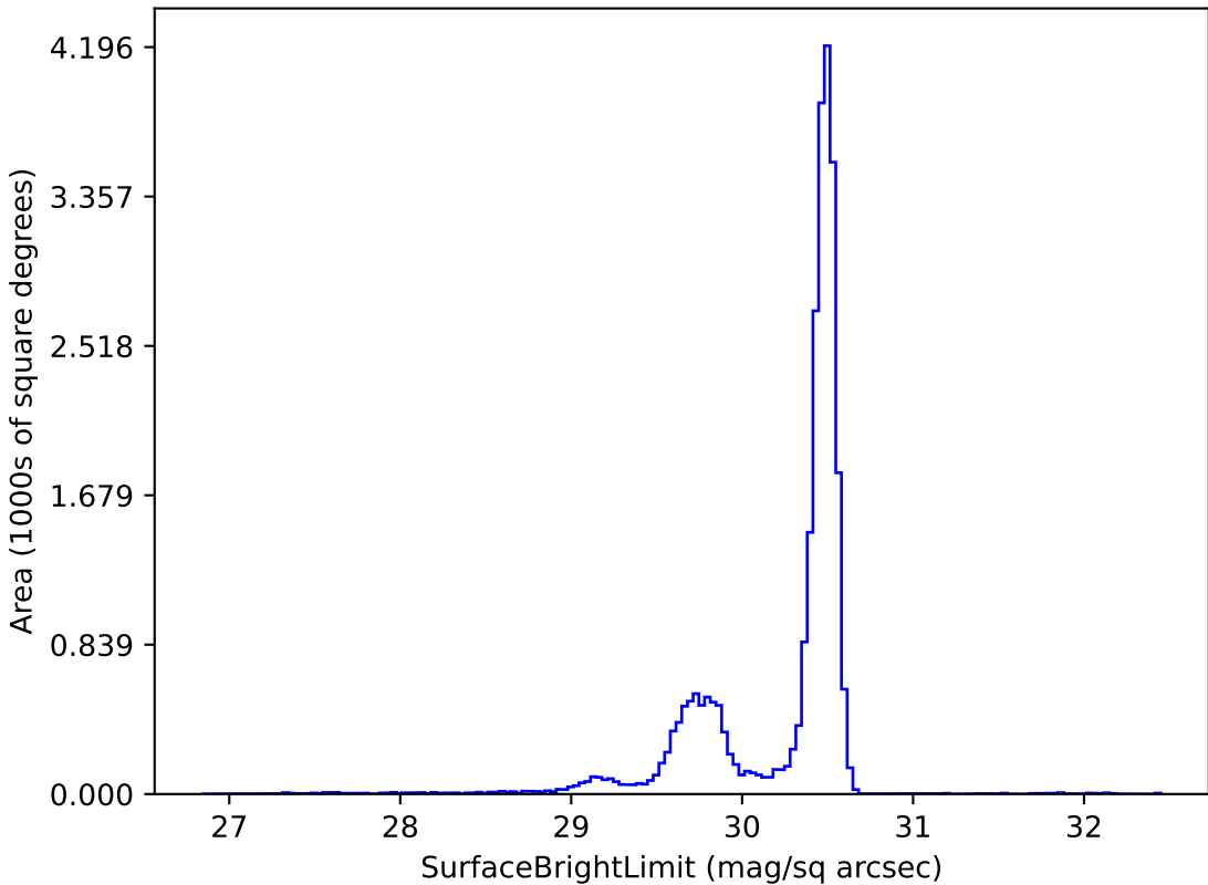
ddf_loaded_half_fl4_v3.4_10yrs r: SurfaceBrightLimit
