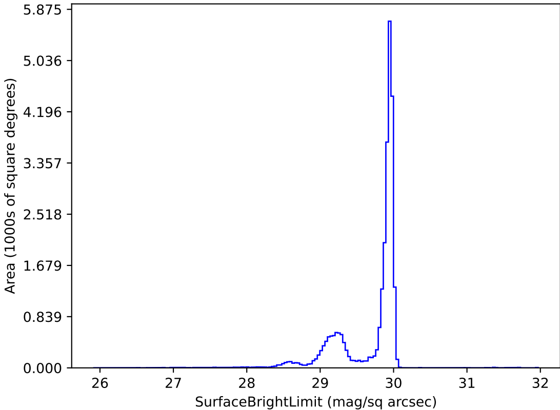
ddf_loaded_half_fl4_v3.4_10yrs i: SurfaceBrightLimit
