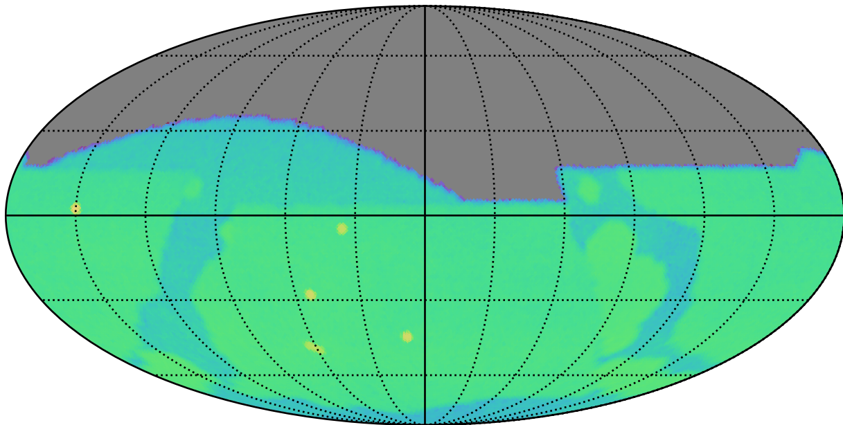
ddf_loaded_half_fl4_v3.4_10yrs g: SurfaceBrightLimit
