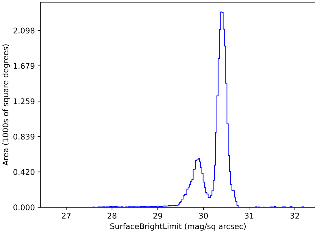
ddf_loaded_half_fl4_v3.4_10yrs g: SurfaceBrightLimit
