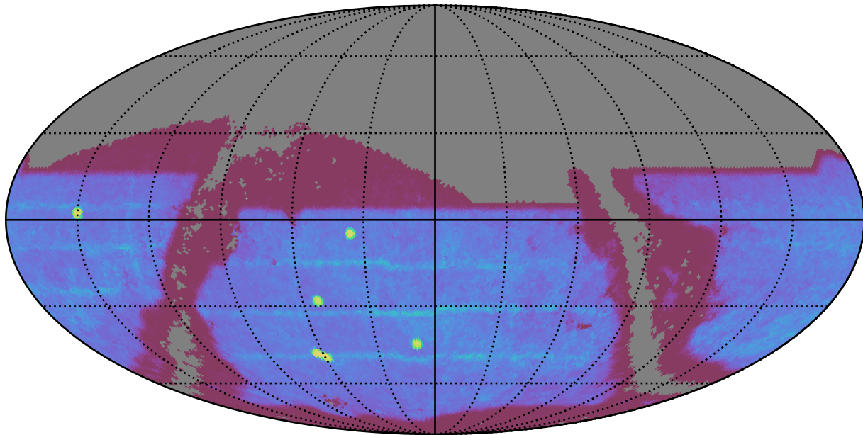
ddf_loaded_half_fl4_v3.4_10yrs : SNSLMetric
