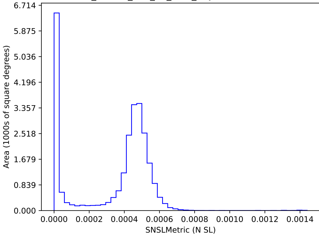
ddf_loaded_half_fl4_v3.4_10yrs : SNSLMetric
