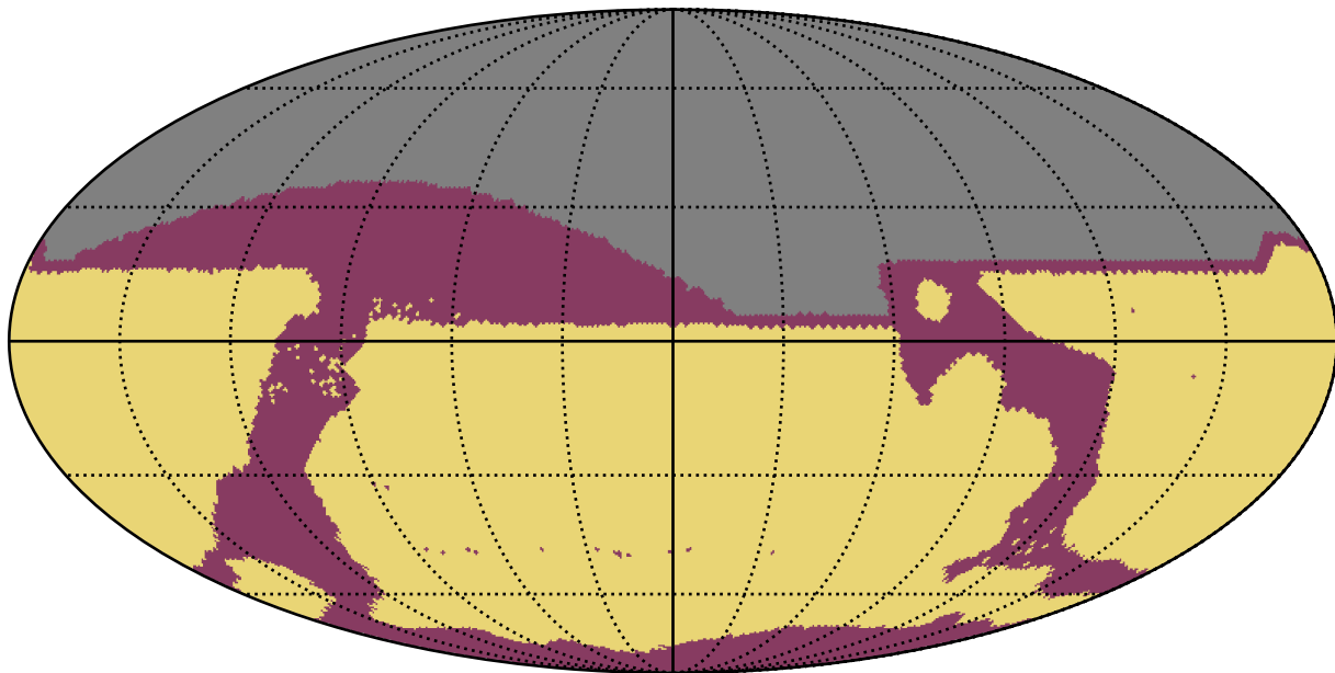
ddf_loaded_half_fl4_v3.4_10yrs : RapidRevisits
