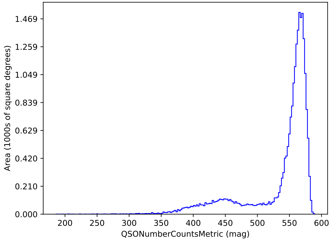
ddf_loaded_half_fl4_v3.4_10yrs y band and non-DD: QSONumberCountsMetric
