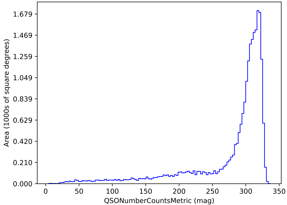
ddf_loaded_half_fl4_v3.4_10yrs u band and non-DD: QSONumberCountsMetric
