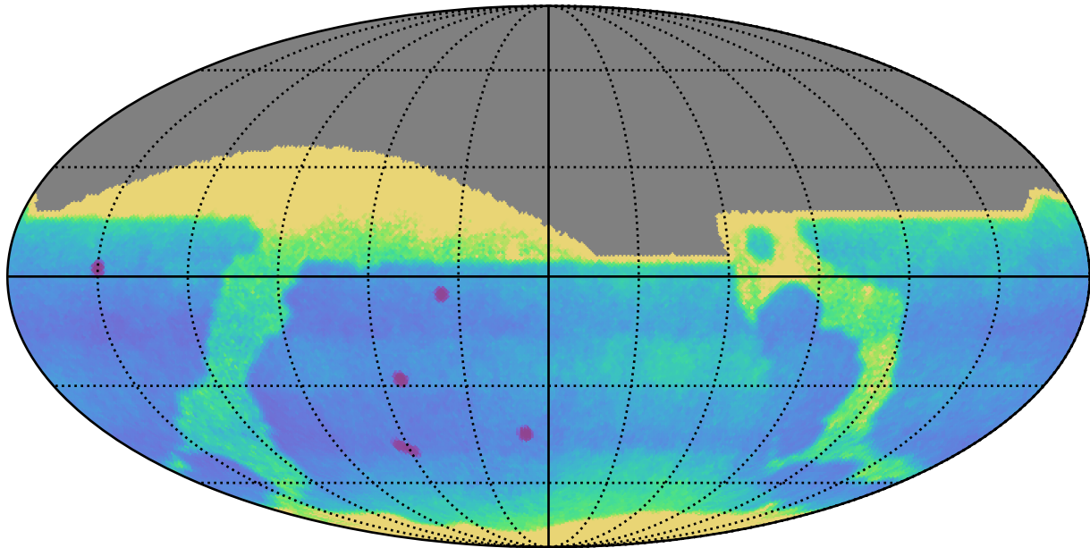
ddf_loaded_half_fl4_v3.4_10yrs : Proper Motion Uncert @ 24.0
