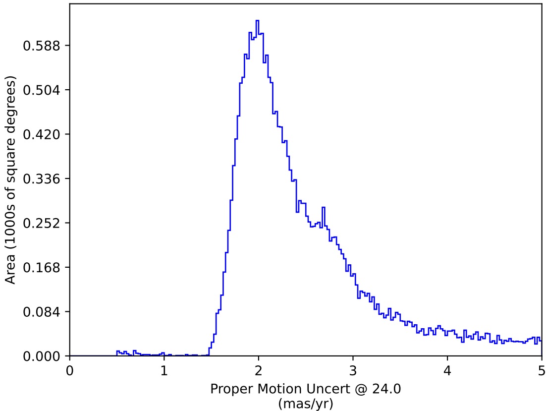
ddf_loaded_half_fl4_v3.4_10yrs : Proper Motion Uncert @ 24.0
