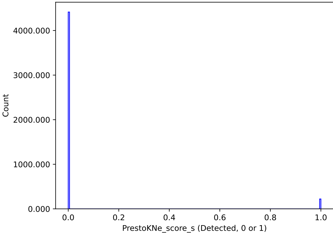
ddf_loaded_half_fl4_v3.4_10yrs : PrestoKNe_score_s
