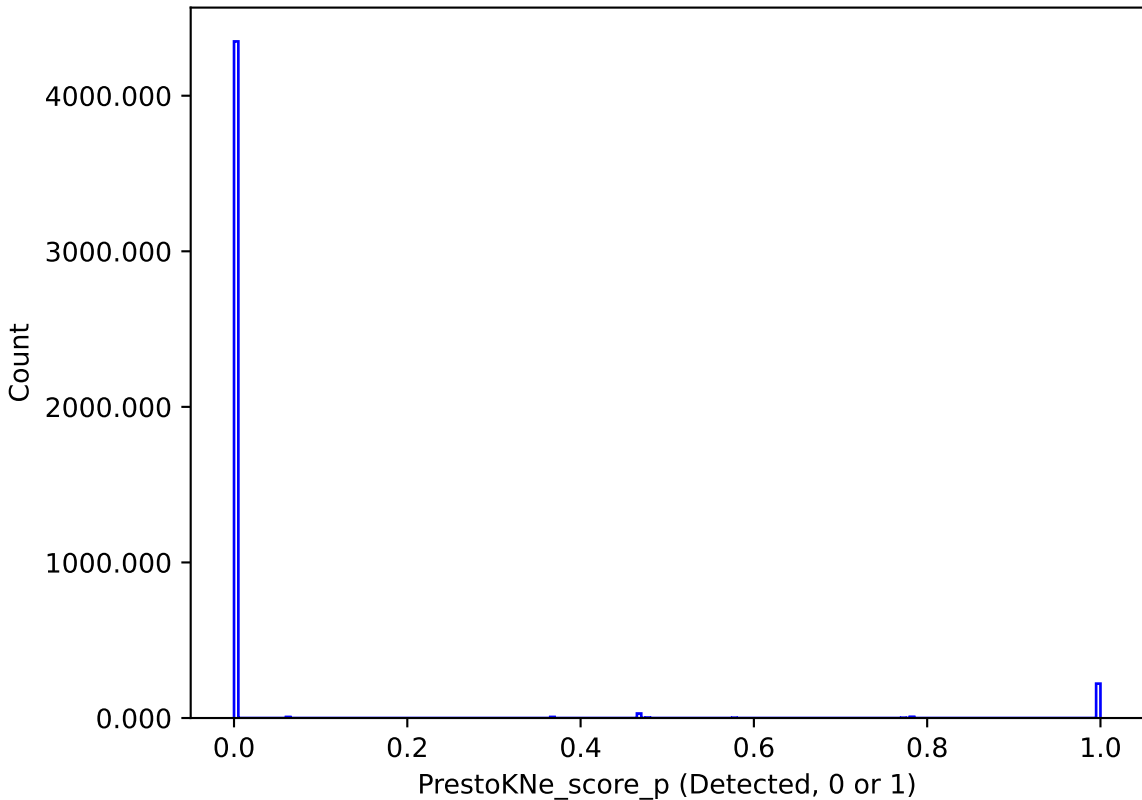
ddf_loaded_half_fl4_v3.4_10yrs : PrestoKNe_score_p
