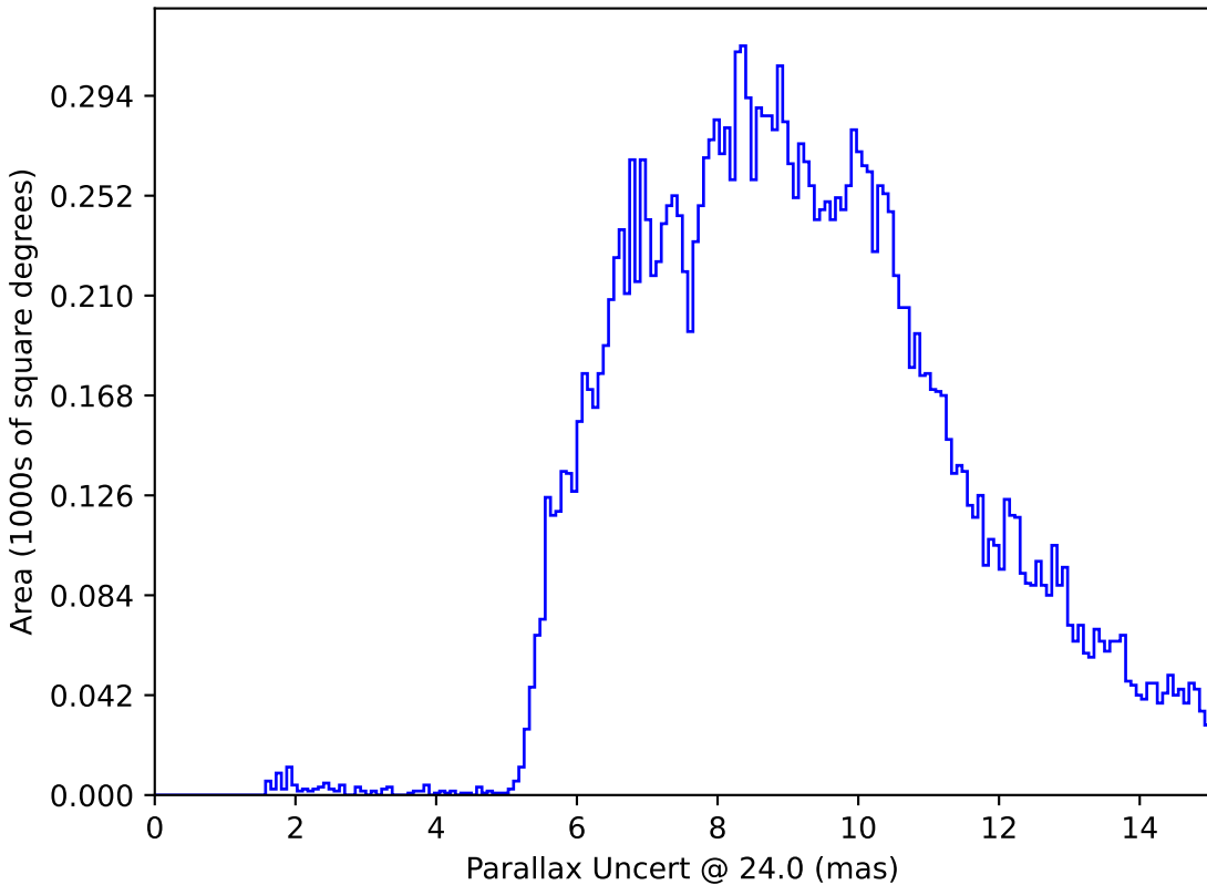
ddf_loaded_half_fl4_v3.4_10yrs : Parallax Uncert @ 24.0
