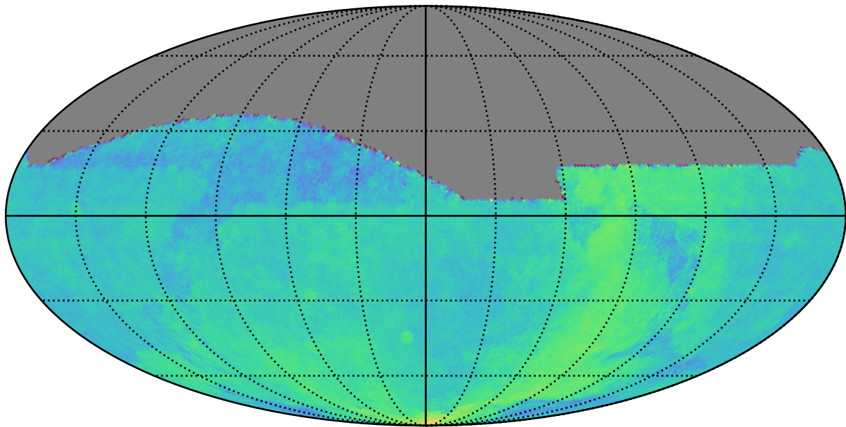
ddf_loaded_half_fl4_v3.4_10yrs : Parallax Coverage @ 24.0
