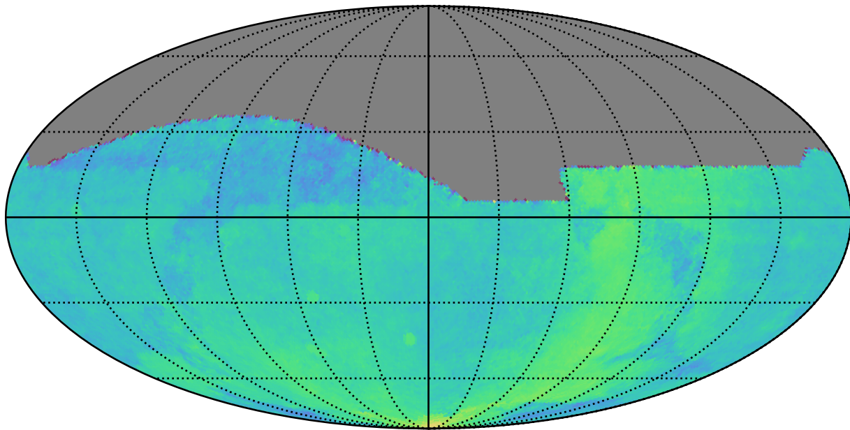
ddf_loaded_half_fl4_v3.4_10yrs : Parallax Coverage @ 22.4
