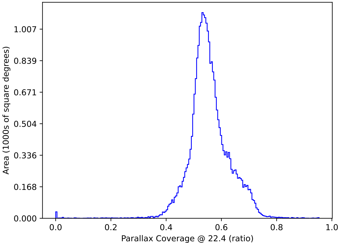
ddf_loaded_half_fl4_v3.4_10yrs : Parallax Coverage @ 22.4
