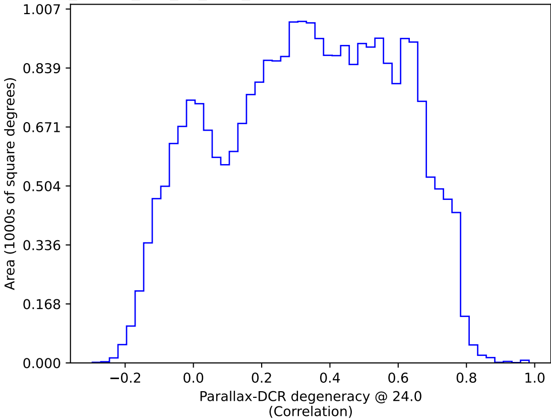
ddf_loaded_half_fl4_v3.4_10yrs : Parallax-DCR degeneracy @ 24.0
