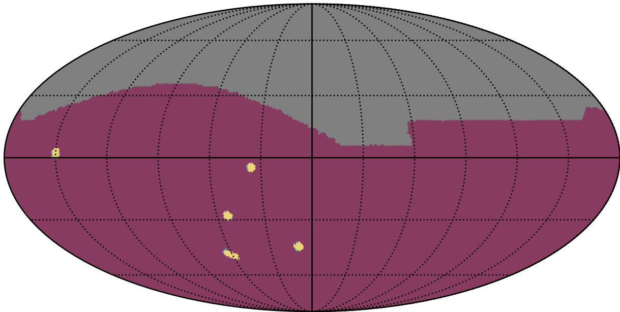
ddf_loaded_half_fl4_v3.4_10yrs : NumberOfQuickRevisits
