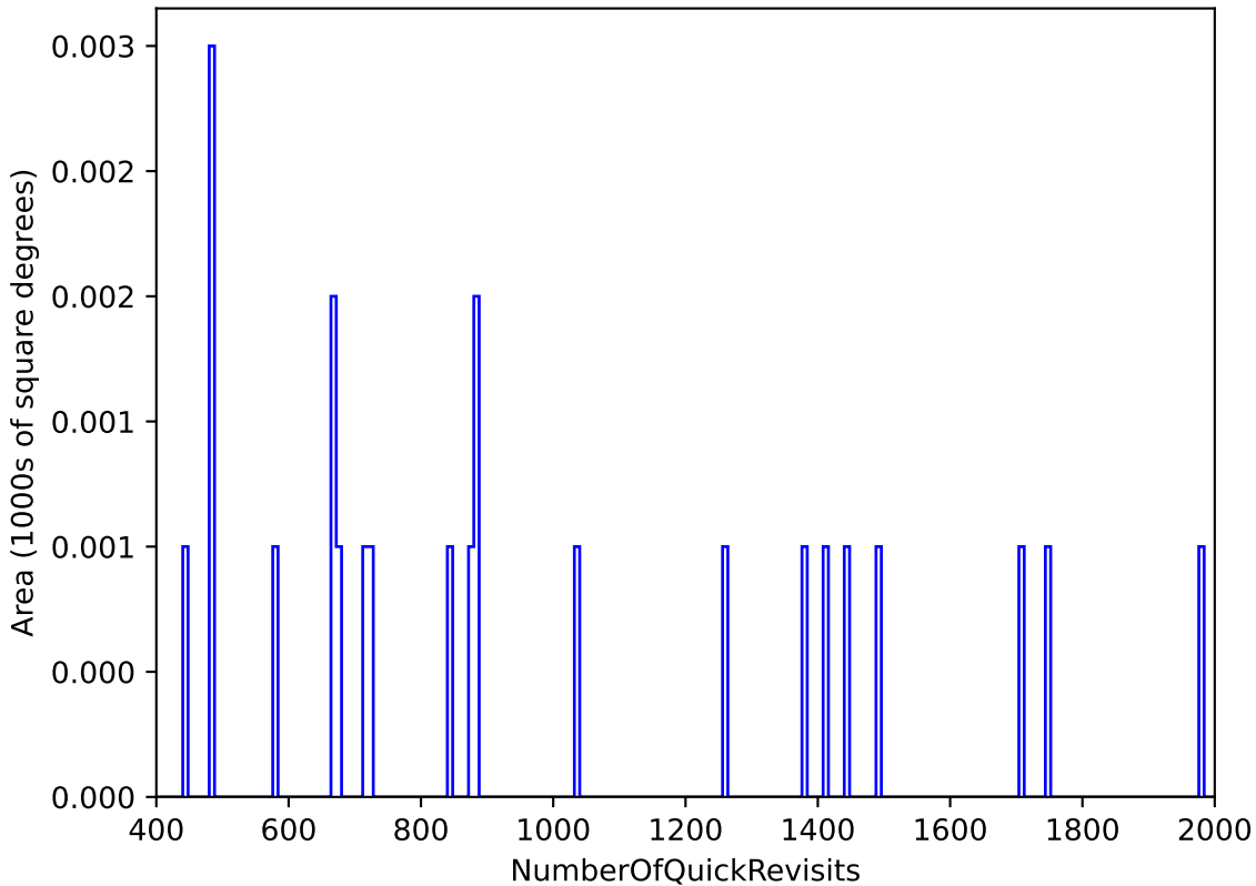
ddf_loaded_half_fl4_v3.4_10yrs : NumberOfQuickRevisits
