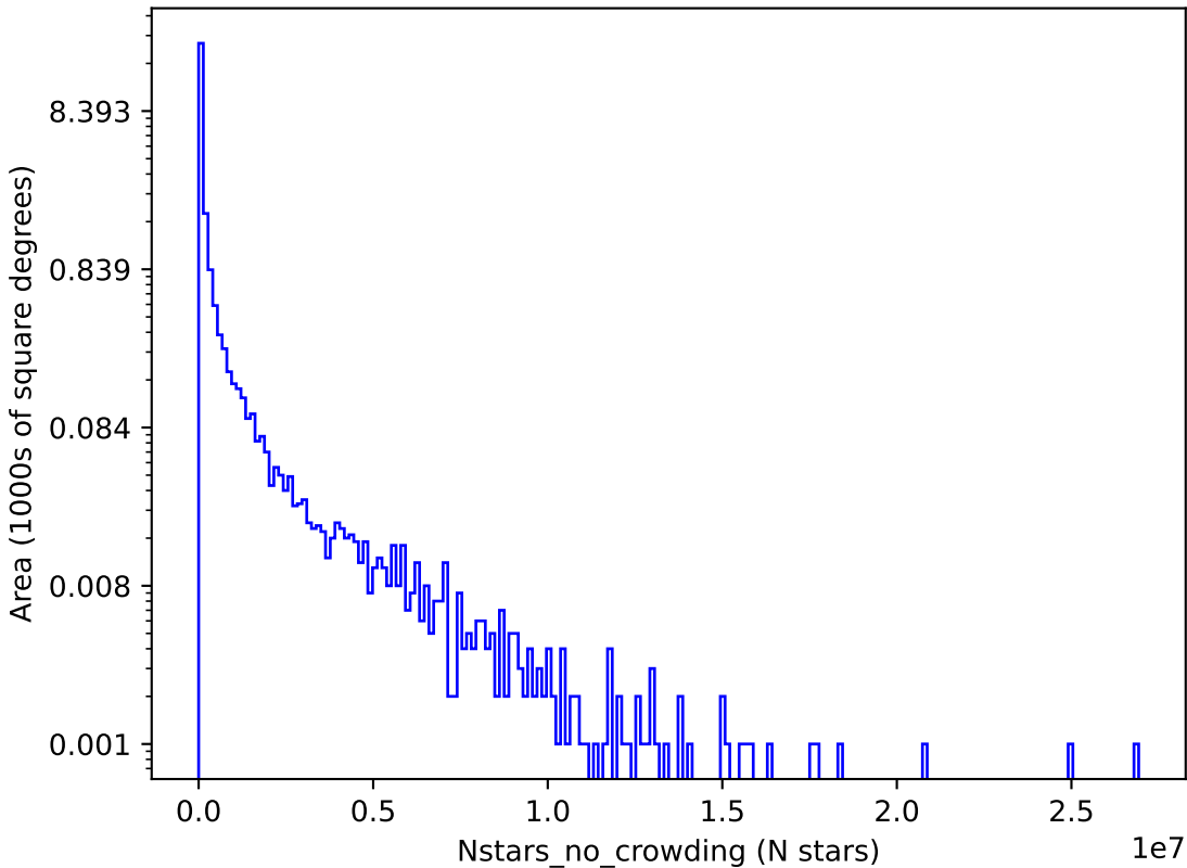
ddf_loaded_half_fl4_v3.4_10yrs z: Nstars_no_crowding
