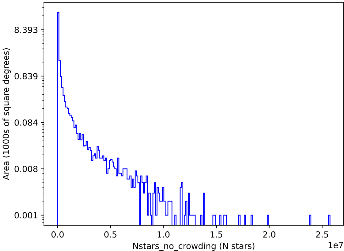
ddf_loaded_half_fl4_v3.4_10yrs y: Nstars_no_crowding
