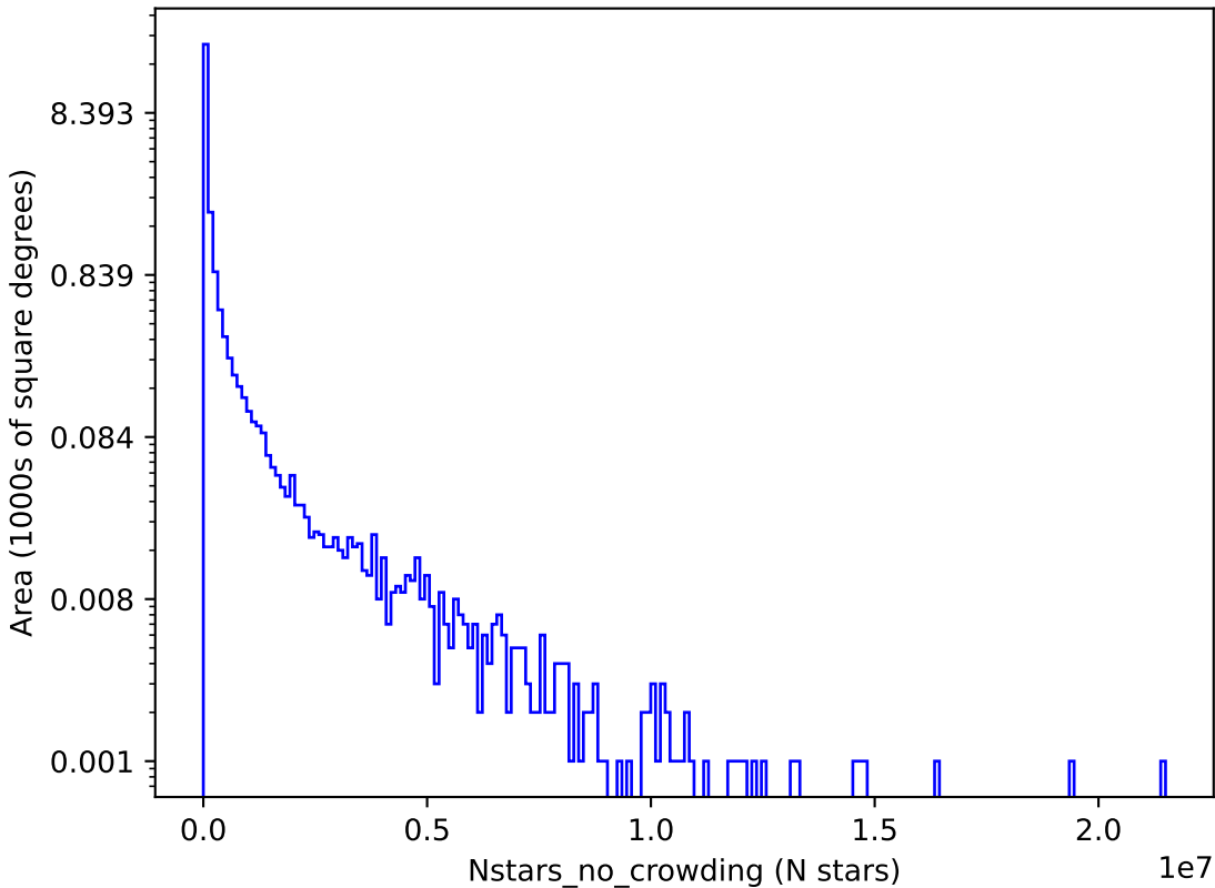
ddf_loaded_half_f14_v3.4_10yrs r: Nstars_no_crowding
