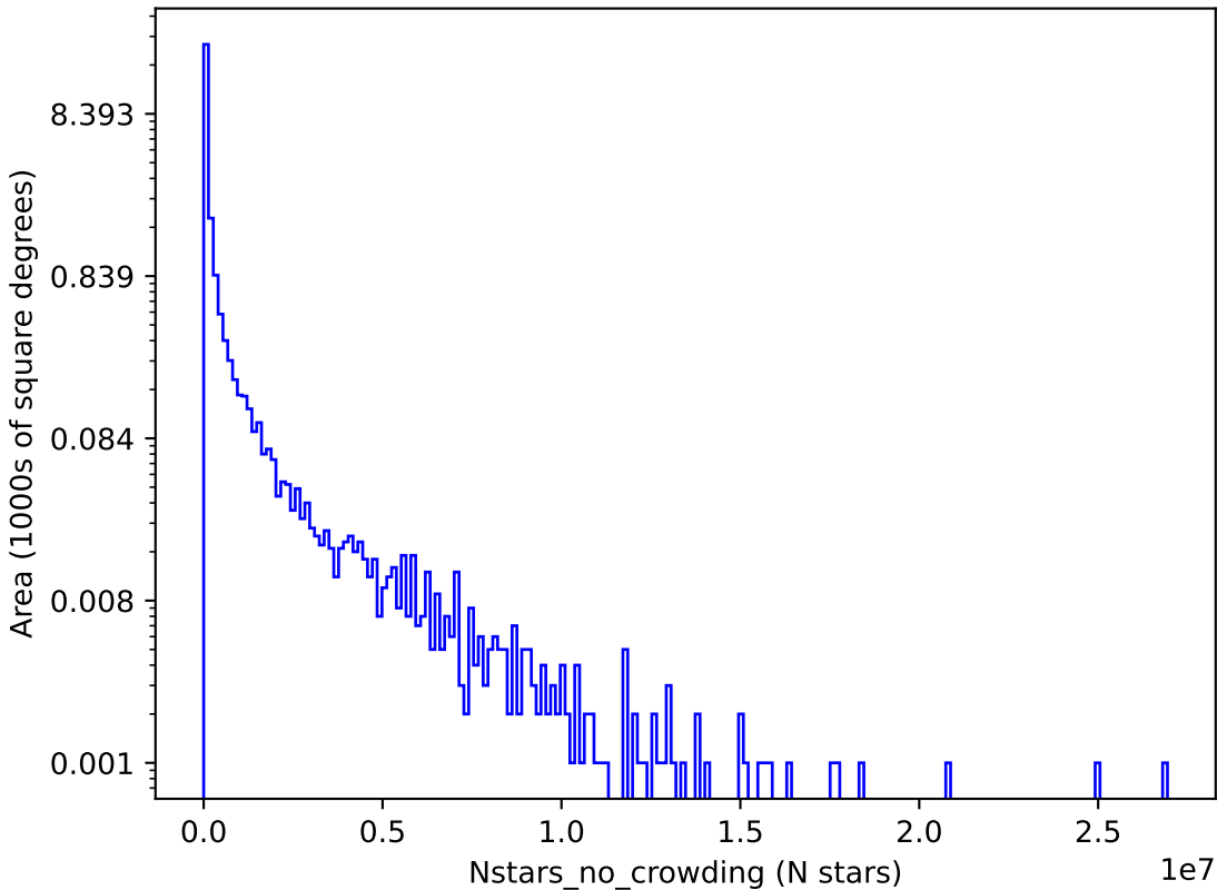
ddf_loaded_half_f14_v3.4_10yrs i: Nstars_no_crowding
