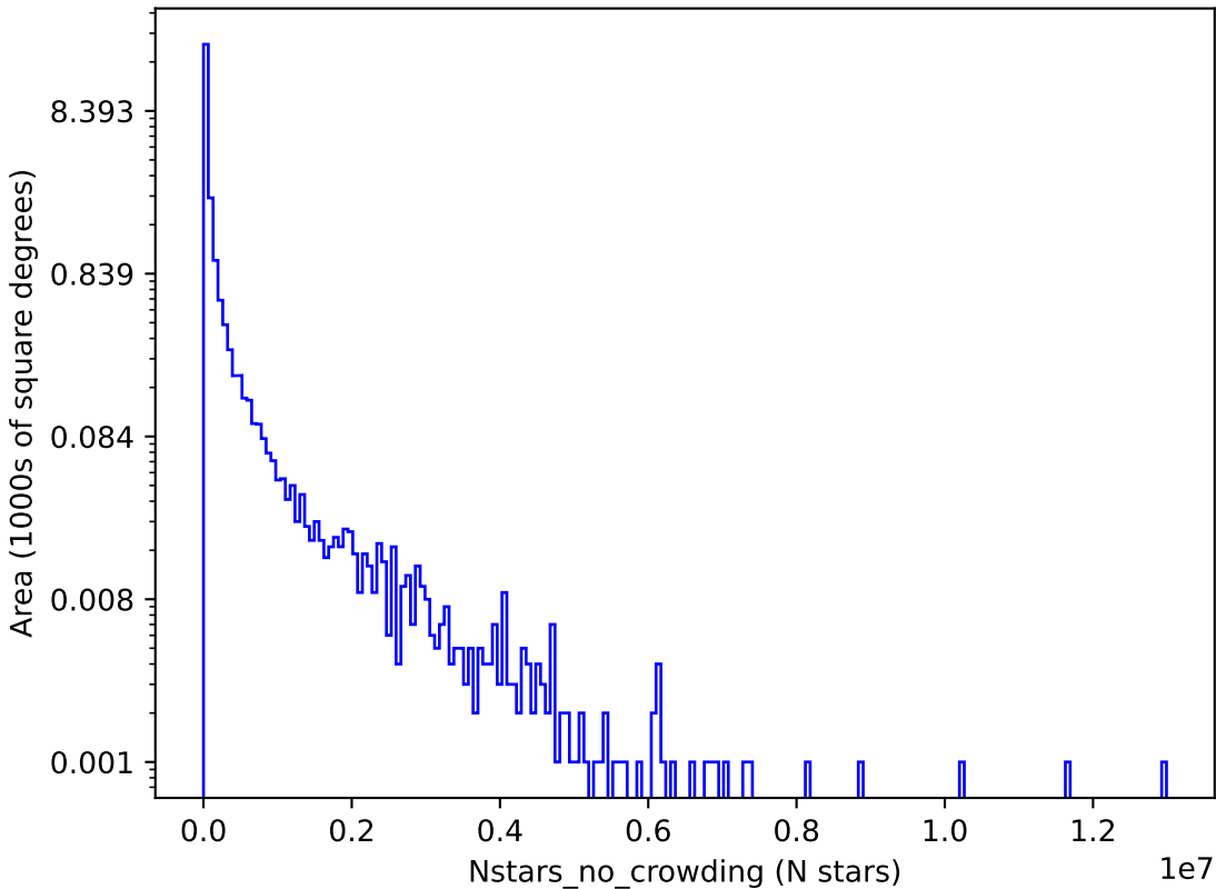
ddf_loaded_half_fl4_v3.4_10yrs g: Nstars_no_crowding
