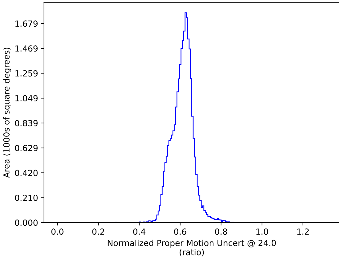
ddf_loaded_half_fl4_v3.4_10yrs : Normalized Proper Motion Uncert @ 24.0
