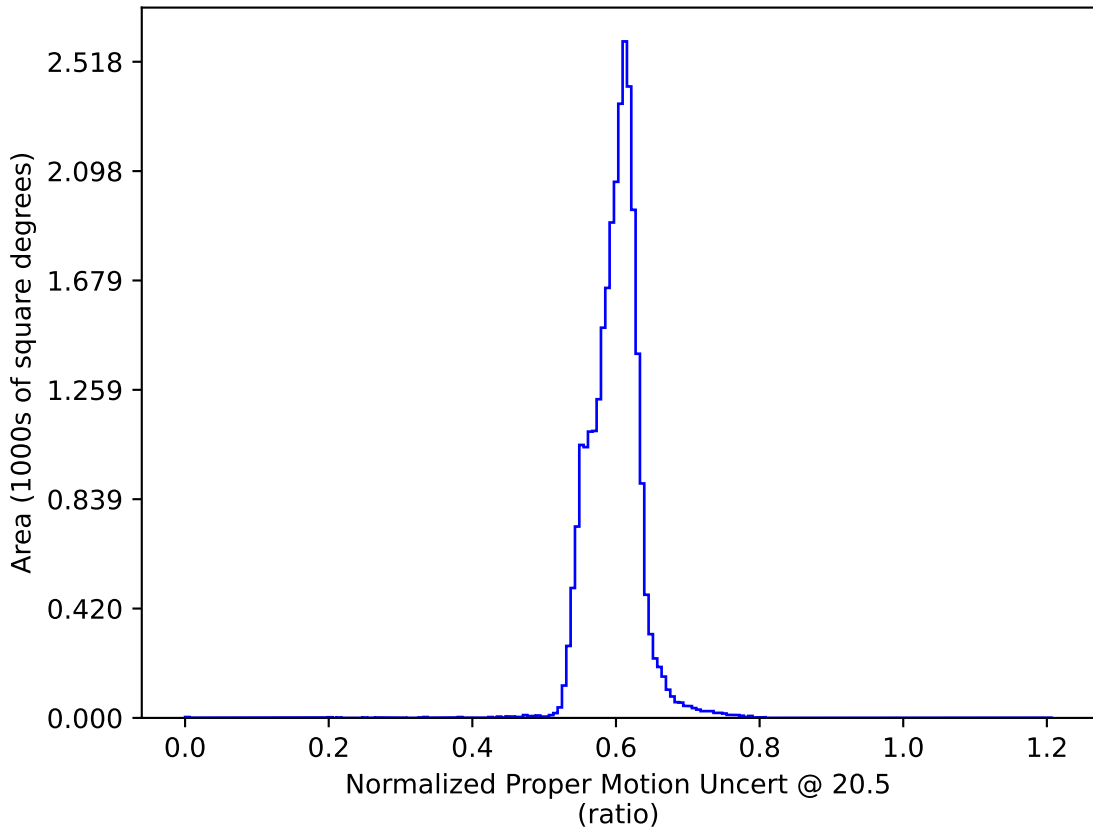
ddf_loaded_half_fl4_v3.4_10yrs : Normalized Proper Motion Uncert @ 20.5
