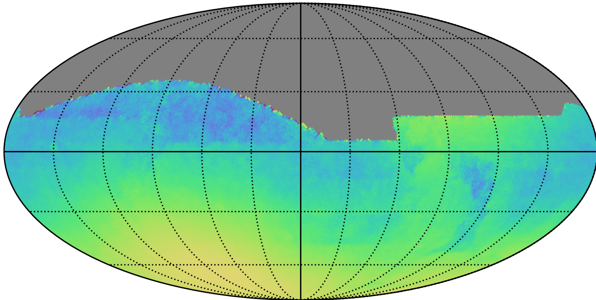
ddf_loaded_half_fl4_v3.4_10yrs : Normalized Parallax Uncert @ 24.0
