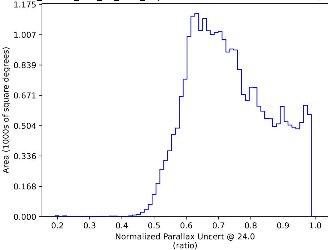
ddf_loaded_half_fl4_v3.4_10yrs : Normalized Parallax Uncert @ 24.0
