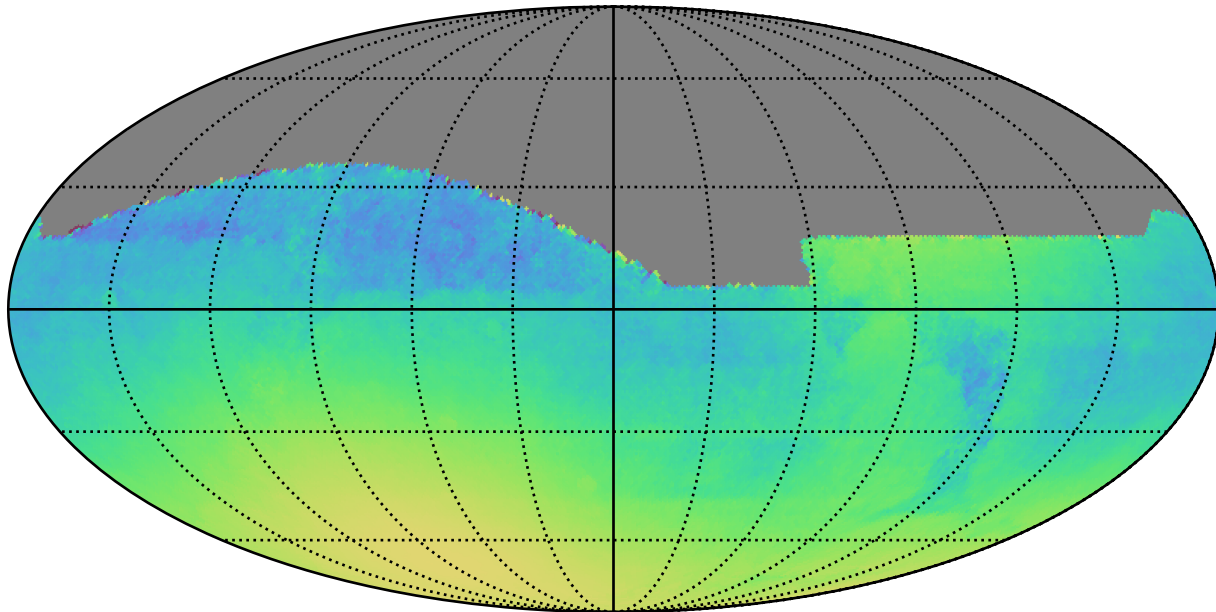
ddf_loaded_half_fl4_v3.4_10yrs : Normalized Parallax Uncert @ 22.4
