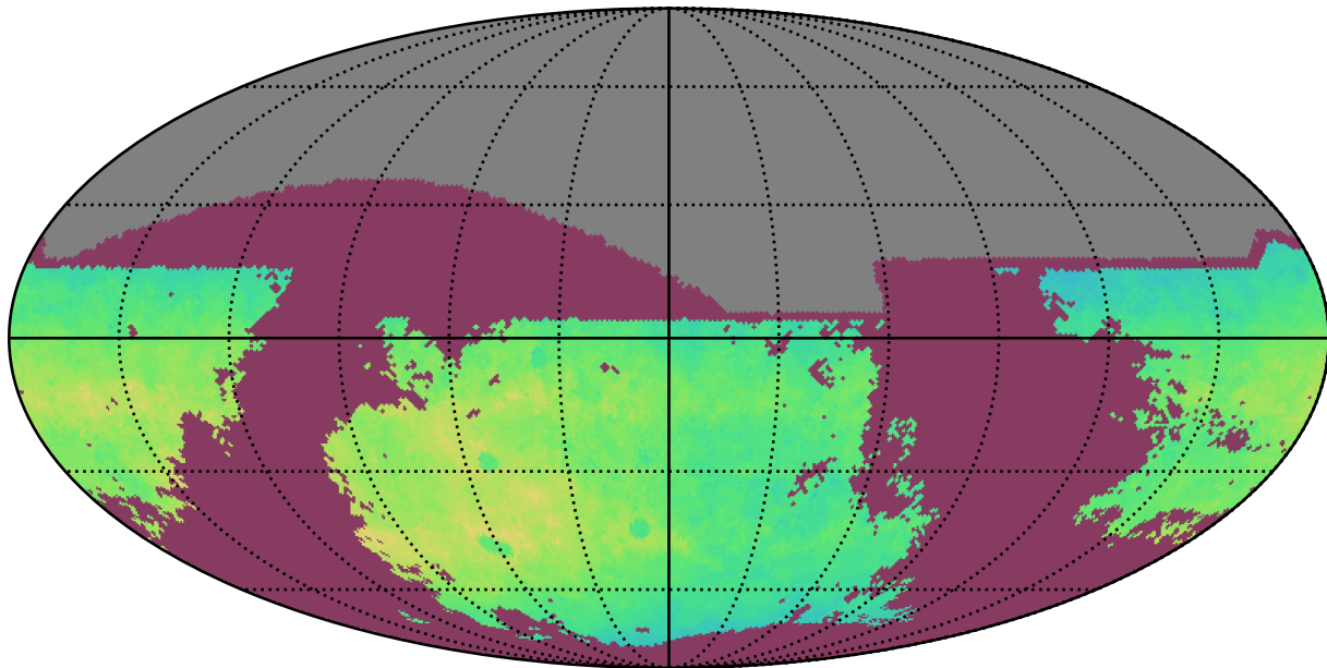
ddf_loaded_half_fl4_v3.4_10yrs i: NgalScale
