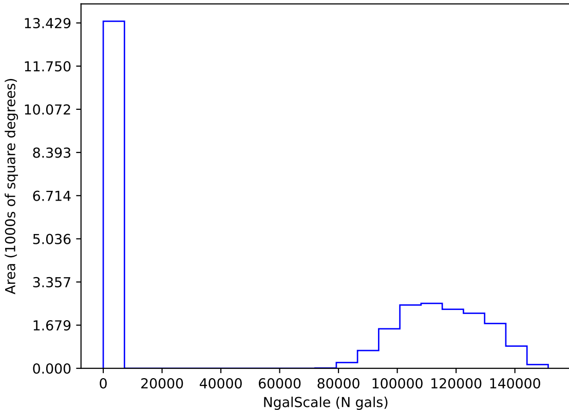
ddf_loaded_half_fl4_v3.4_10yrs i: NgalScale
