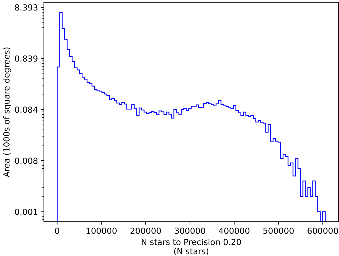
ddf_loaded_half_f14_v3.4_10yrs y: N stars to Precision 0.20
