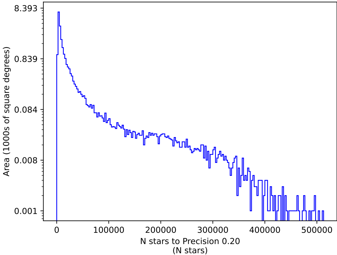
ddf_loaded_half_f14_v3.4_10yrs u: N stars to Precision 0.20
