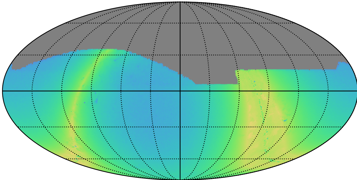
ddf_loaded_half_fl4_v3.4_10yrs i: N stars to Precision 0.20
