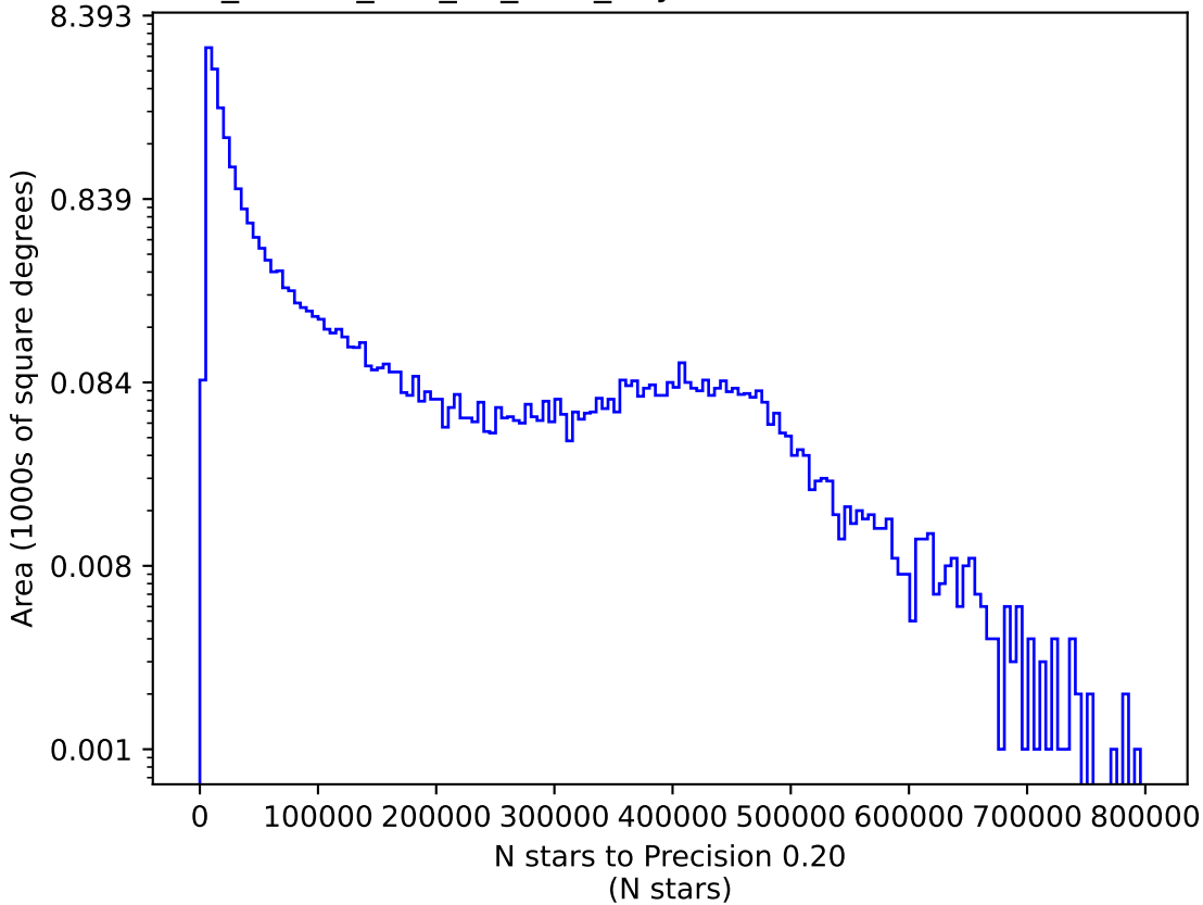
ddf_loaded_half_fl4_v3.4_10yrs i: N stars to Precision 0.20
