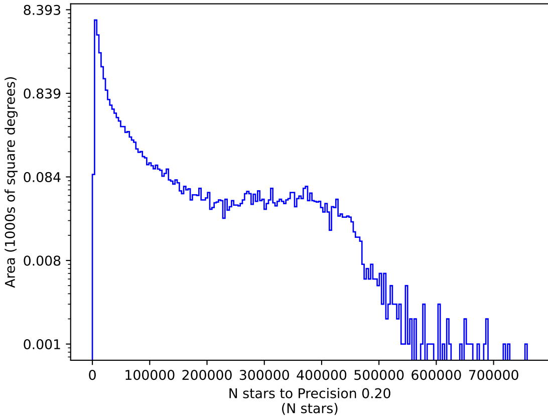
ddf_loaded_half_fl4_v3.4_10yrs g: N stars to Precision 0.20
