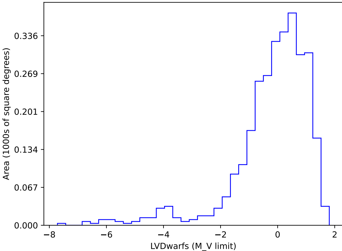
ddf_loaded_half_fl4_v3.4_10yrs gi SCP: LVDwarfs
