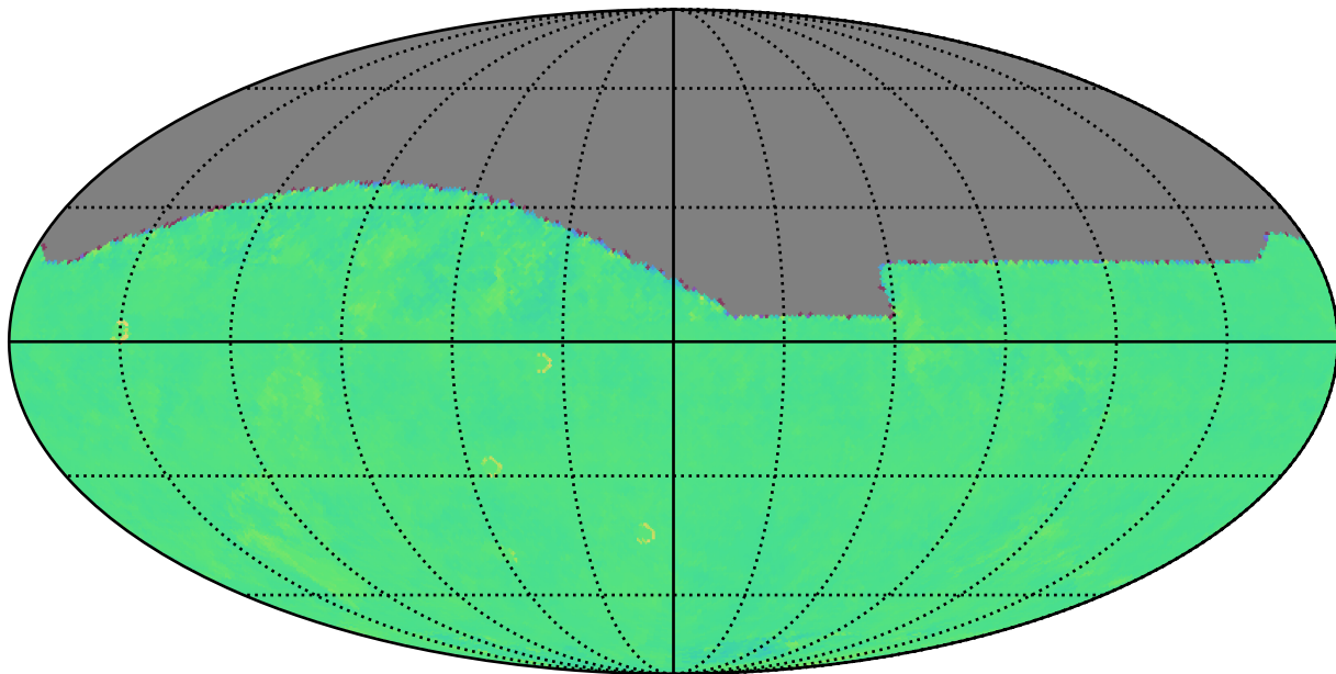
ddf_loaded_half_fl4_v3.4_10yrs z: Kuiper rotTelPos
